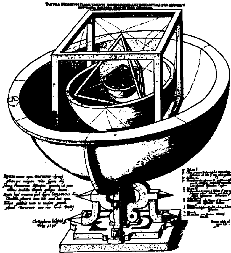
FIGURE 3. Kepler's model of the organization of the solar system according to the Platonic Solids (left), with a modern reconstruction (below).
