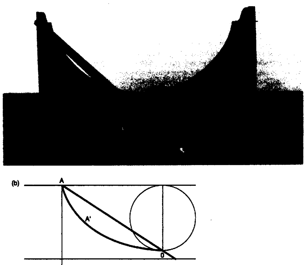
FIGURE 4. The principle of isochronism. (a) Model: inverted cycloid and straight-line raceways for rolling balls. A two-channel cycloid raceway enables comparison of the times for balls released simultaneously from different starting positions (A, A') to reach the bottom of the curved track, as shown in diagram (b).
